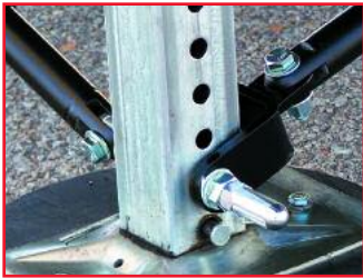
JT's Strong Arm Jack Stabilizers connected to an electric jack
